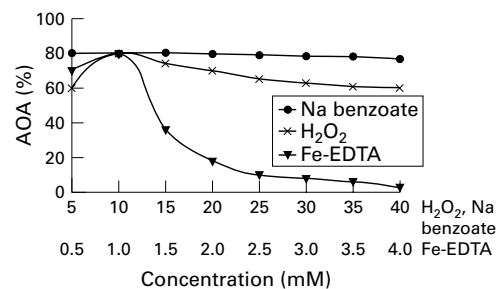
Figure 1 Influence of the concentration of reagents on antioxidant activity (AOA). Na benzoate was used at 5–40 mM (while Fe-EDTA was kept at 1 mM and \text{H}_2\text{O}_2 at 10 mM). \text{H}_2\text{O}_2 was used at 5–40 mM (while Fe-EDTA was kept at 1 mM and Na benzoate at 10 mM). Fe-EDTA was used at 0.5–4 mM (while \text{H}_2\text{O}_2 was kept at 10 mM and Na benzoate at 10 mM).
