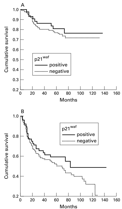
Figure 2 Kaplan-Meier curves for disease free survival (event = relapse) for (A) node negative (n = 130) and (B) node positive (n = 159) subgroups. Only trends could be observed (log rank test: p > 0.05 ).
