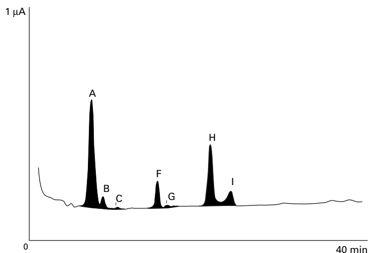
Figure 2 Chromatogram of oligosaccharides of IgG from a patient with stage III myeloma. Neutral oligosaccharides are represented by peaks A, B, and C; monosialylated forms are represented by peaks F and G; disialylated form are represented by peaks H and I. There is a large increase in the proportion of disialylated oligosaccharides in this sample.
