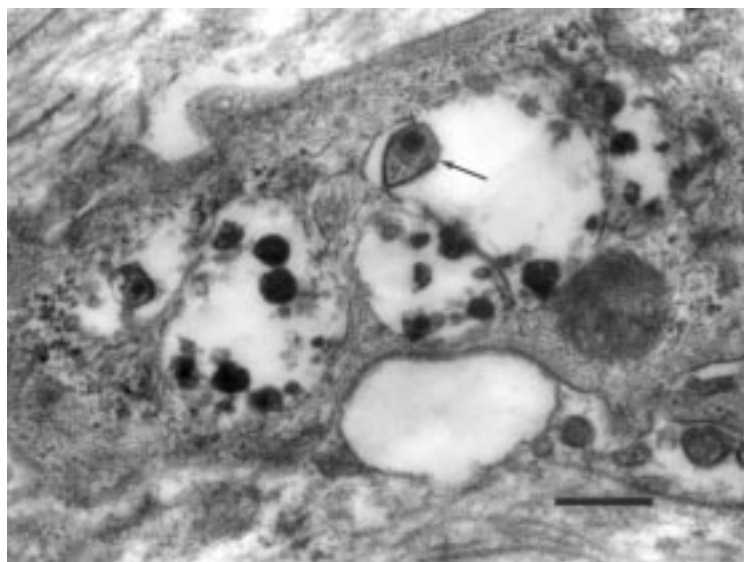
Figure 1 Transmission electron micrograph of an atheromatous arterial wall. Elementary bodies of Chlamydia pneumoniae in vacuoles within a smooth muscle cell. The organisms appear pear shaped in some profiles (arrowed) and contain a central, electron-dense core. The scale bar represents 300 nm.
